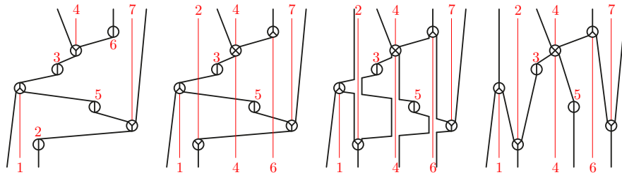
Figure 13. Refinement by cut and stretch: starting from a permutree decorated with \sigma (left), we redecorate its vertices with \tau (middle left), cut and reconnect its edges along the resulting red walls (middle right), and stretch the resulting \tau -permutree (right).
