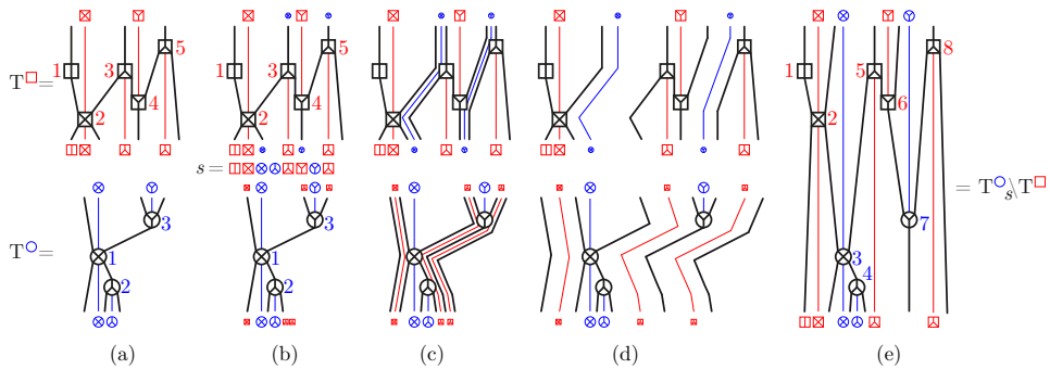
Figure 18. (a) The two initial permutrees T^\square and T^\circ . (b) Given the shuffle s = \square\square\square\square\square\square\square\square , the positions of the \square and \circ are reported in T^\square and the positions of the \square and \circ are reported in T^\circ . (c) The corresponding laminations. (d) The permutrees are split according to the laminations. (e) The resulting permutree T^\square \setminus_s T^\circ .
