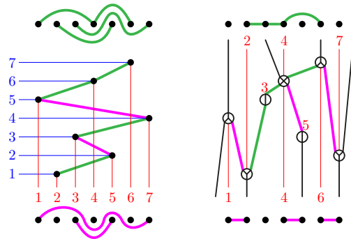
Figure 7. The arc diagrams \text{asc}(\sigma) (green, up) and \text{desc}(\sigma) (pink, down) associated to the permutation \sigma = 2537146 (left) and the arc diagrams \text{asc}(T) (green, up) and \text{desc}(T) (pink, down) associated to a permutree T (right).
