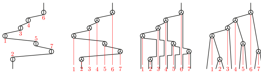
Figure 14. BST insertion seen as the refinement map from a \tau -permutree (i.e. a permutation of \mathfrak{S}_n ) to a \tau -permutree (i.e. a binary tree on [n] ).
