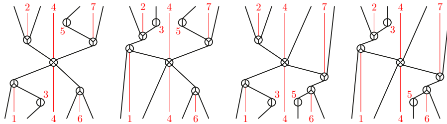
Figure 20. The four generators of the upper ideal of E-indecomposable \bar{\sigma} -permutrees for the decoration \bar{\sigma} = \dots
