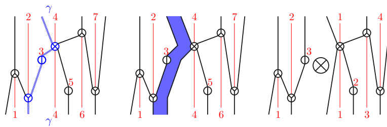
Figure 19. A gap \gamma between 3 and 4 (left) defines a vertical cut (middle) which splits the permutree vertically (right).
