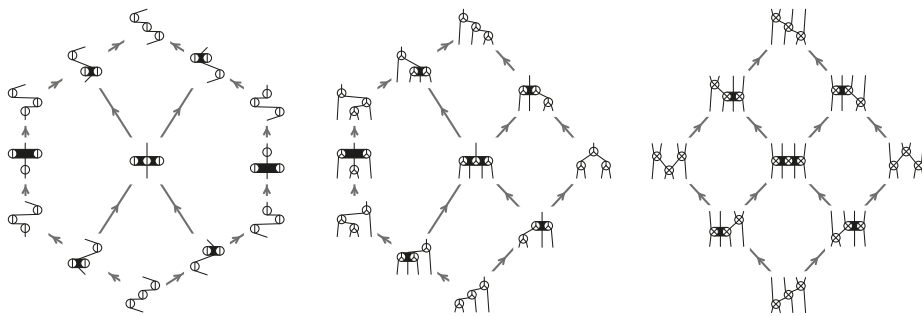
Figure 25. The Schröder -permutree lattices for n = 3 (left), 3 (middle) and 3 (right).
