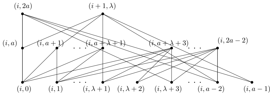
FIGURE 14. P \setminus (S_i \cup S_{i+1}) in case (6.2).
