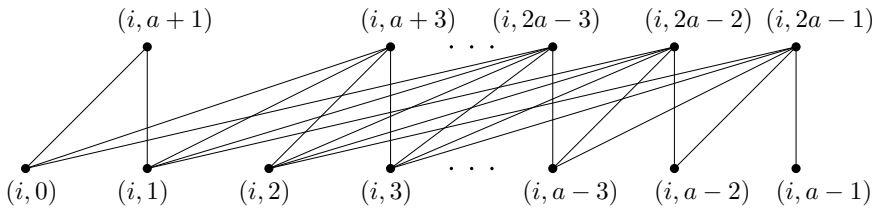
FIGURE 11. P \setminus S_i in case (4) for x = a + 2 .
