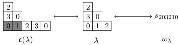
FIGURE 1. k = 3 , \lambda = (3, 2, 1) \in \mathcal{P}_3 , \mathbf{c}(\lambda) = (5, 2, 1) \in \mathcal{C}_4 , and w_\lambda = s_{203210} \in \tilde{S}_4^\circ .
