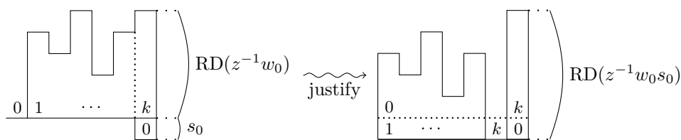
FIGURE 6. Inserting s_0 into \text{RD}(z^{-1}w_0) and justify it to obtain a k -code for z^{-1}w_0s_0 .
