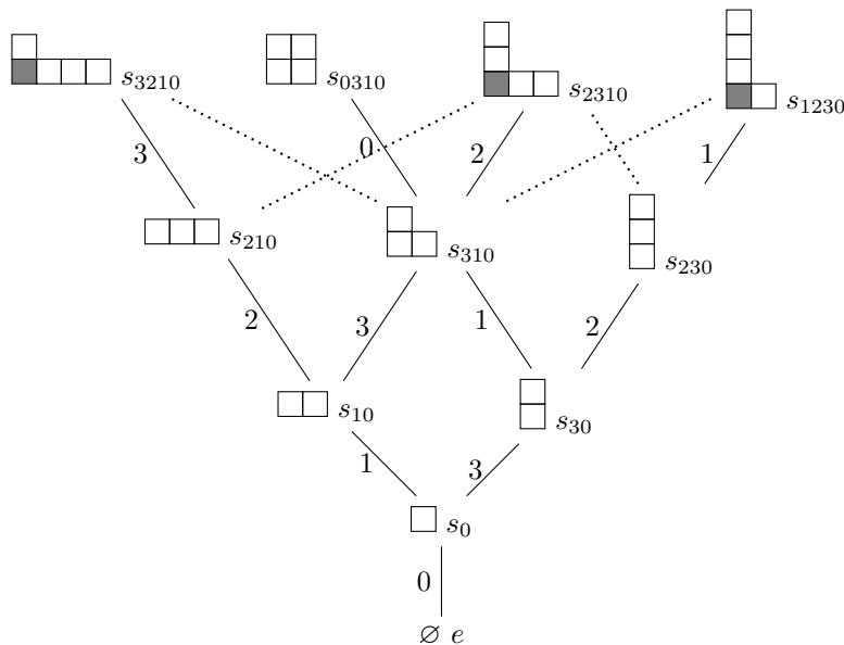
FIGURE 9. The poset of 4-cores (and corresponding elements in \widetilde{S}_4^\circ ) up to those of size 4. The left weak covers are represented by solid lines, and the strong covers are dotted or solid lines. A solid edge labelled with i corresponds to the left multiplication by s_i .
