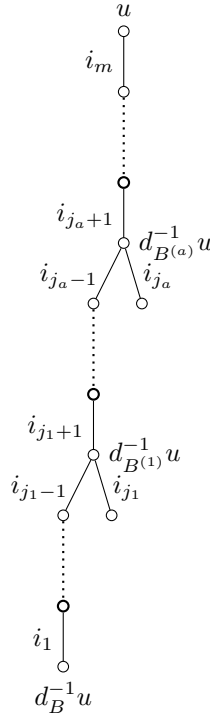
FIGURE 14. For Lemma 5.12
