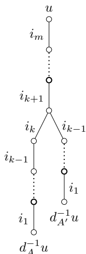
FIGURE 13. For Lemma 5.11
