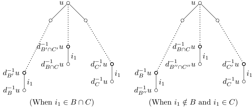
FIGURE 12. For Lemma 5.7
