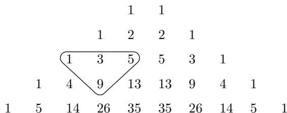
FIGURE 1. Generalized Pascal triangle generating the numbers N_{n,\ell} : each entry is the sum of the three entries above it: for instance, we find N_{5,2} = 9 = 1 + 3 + 5 = N_{4,0} + N_{4,1} + N_{4,2} ; missing values are 0.
