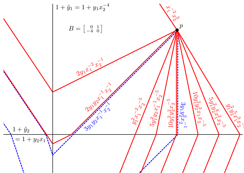
FIGURE 5. Computing \vartheta_{-2\rho_1+3\rho_2} for a = -4 and b = 1
