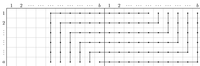
FIGURE 2. A facet in \Delta_7 with a = 6, b = 10
