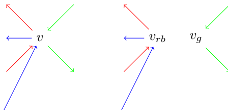
FIGURE 1. Before and after splitting an X -regular graph, with X = \{\text{red, green, blue}\} , at a vertex v along Y = \{r, b\}
