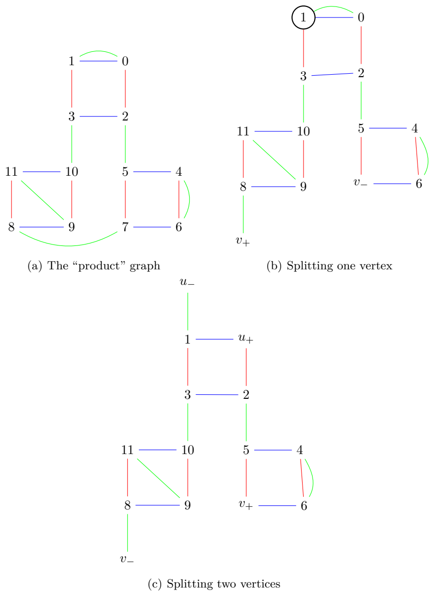
FIGURE 4. The “link” graphs for T = \mathbb{Z}_2 * \mathbb{Z}_2 * \mathbb{Z}_2 : (a) the original graph; (b) the result of splitting 7; (c) the result of splitting 0 and 7. The root of the edge link is encircled.
