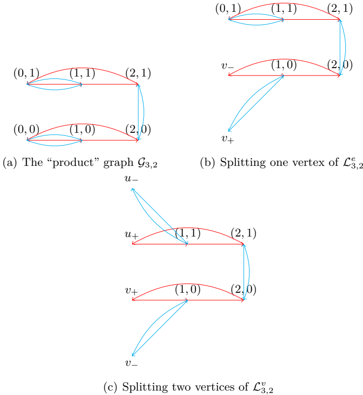
FIGURE 2. The “link” graphs for T = \mathbb{Z}_3 * \mathbb{Z}_2 : (a) the original graph; (b) the result of splitting (0,0) ; (c) the result of splitting (0,0) and (0,1) . The root of the edge link is (0,1) .
