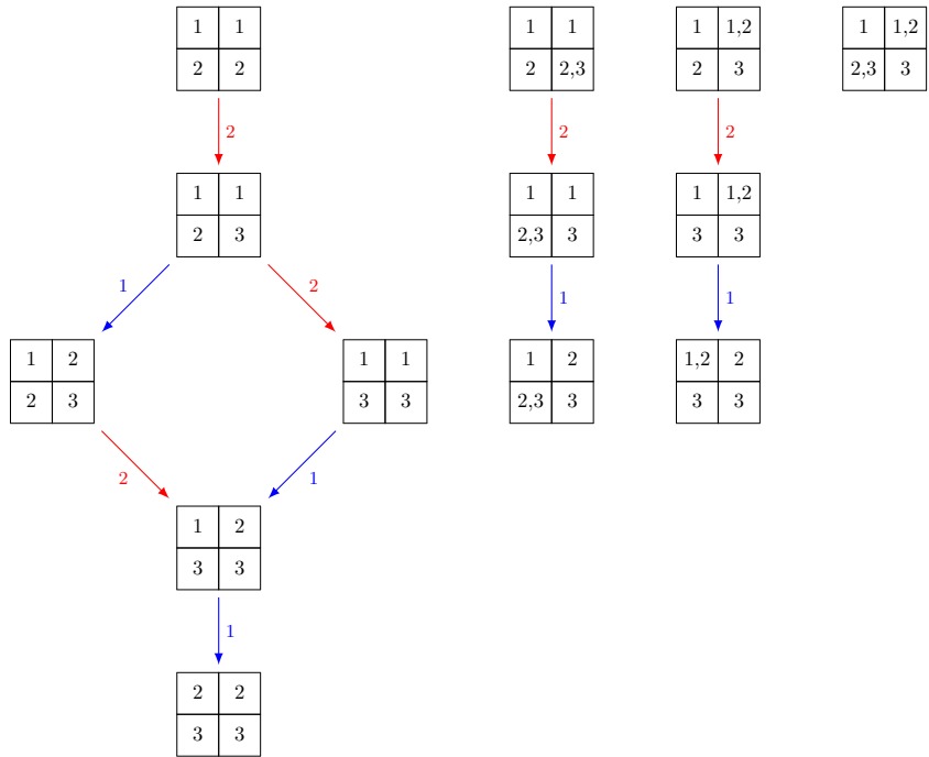
FIGURE 1. The U_q(\mathfrak{sl}_3) -crystal structure on \text{SVT}^3\left(\begin{smallmatrix} \square & \square \\ \square & \square \end{smallmatrix}\right) . An i -arrow b \xrightarrow{i} b' represents the action of the crystal operator f_i b = b' .
