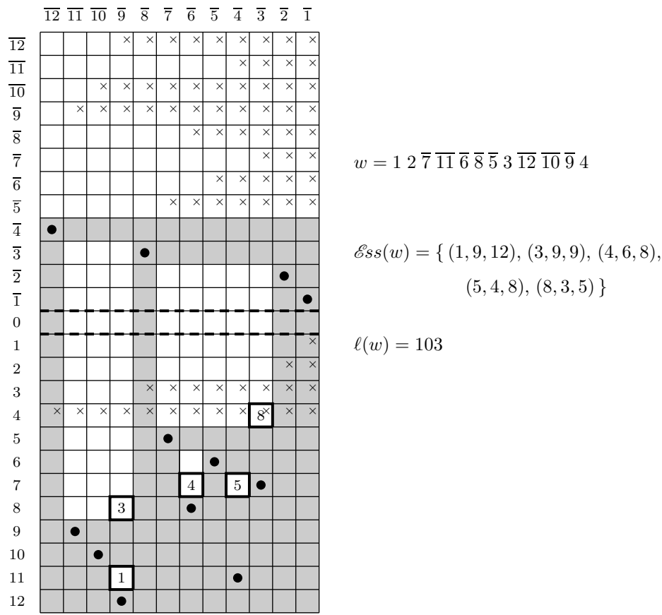
FIGURE 2. Diagram and essential set of a signed permutation. (This is also the vexillary signed permutation for the triple \tau = (1\ 3\ 4\ 5\ 8, 9\ 9\ 6\ 4\ 3, 12\ 9\ 8\ 8\ 5) .)
