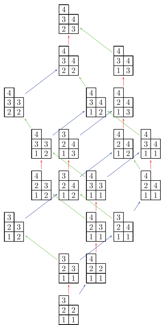
FIGURE 3. The crystal B(2, 2, 1) , with edges f_1 \xleftarrow{\text{green}} , f_2 \xrightarrow{\text{red}} , f_3 \xrightarrow{\text{blue}} .
