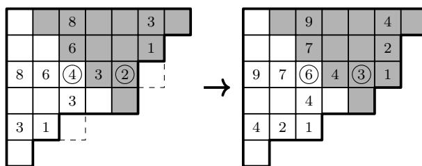
FIGURE 9. The effect of adding a cell on the hook-lengths in a shifted diagram and its double.
