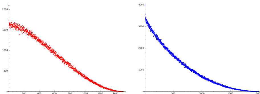
FIGURE 22. The number of occurrences of distances between adjacent entries in a random sorting network of size n = 1500 (left) and a random 132-avoiding sorting network of size n = 2000 (right).
