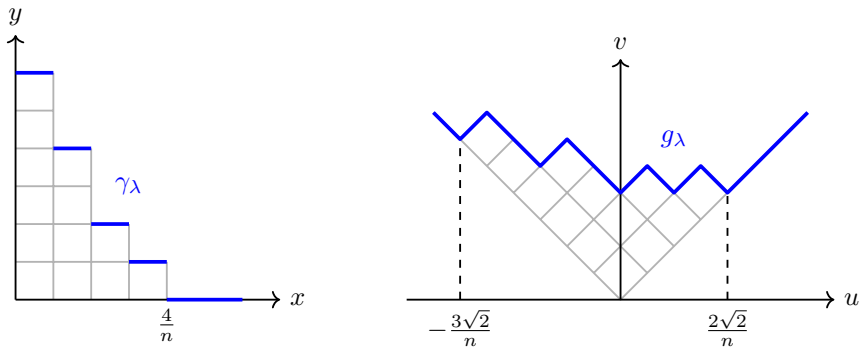
FIGURE 11. The functions \gamma_\lambda and g_\lambda for the partition (6, 4, 2, 1) .
