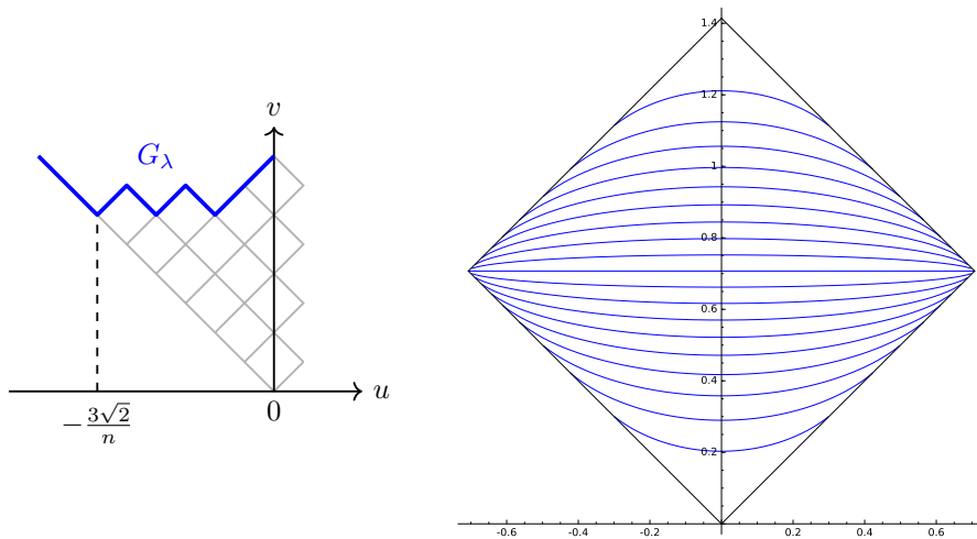
FIGURE 12. Left: the function G_\lambda for the partition (6, 4, 2, 1) . Right: the curves v = g_\alpha(u) for \alpha = 0.05, 0.1, \dots, 0.95 .
