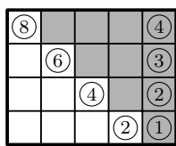
(a) The hook-lengths on the diagonal and in the last column of \Lambda satisfy h_{\Lambda}(i, i) = 2h_{\Lambda}(i, \ell(\lambda) + 1) = 2h_{\lambda}^{\text{sh}}(i, \ell(\lambda)) .
