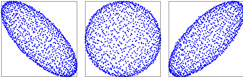
FIGURE 4. The intermediate permutation matrices of \sigma_{[\alpha N]} of a 1000-element random sorting network at times \alpha = \frac{1}{4}, \frac{1}{2} and \frac{3}{4} .
