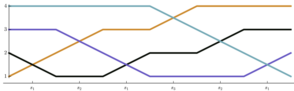
FIGURE 15. Trajectories in the 132-avoiding sorting network 121321. The permutations \sigma_k are \sigma_0 = 1234, \sigma_1 = 2134, \sigma_2 = 2314, \sigma_3 = 3214, \sigma_4 = 3241, \sigma_5 = 3421 and \sigma_6 = 4321 . Hence the trajectory of the element 3 is (3, 3, 2, 1, 1, 1, 2) .
