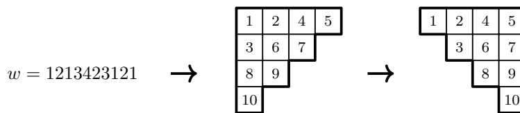
FIGURE 6. The Edelman–Greene correspondence for a 5-element 132-avoiding sorting network.
