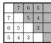
(b) The off-diagonal hook-lengths to the left of the last column of \Lambda satisfy h_{\Lambda}(i, j) = h_{\Lambda}(j, i) = h_{\lambda}^{\text{sh}}(i, j - 1) .
