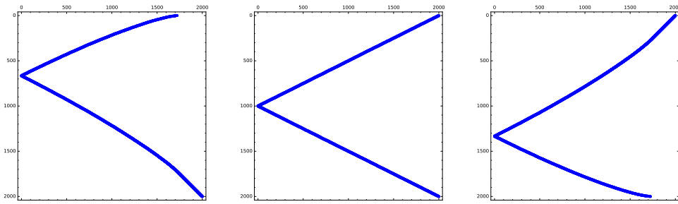
FIGURE 14. The intermediate permutation matrices of a random 132-avoiding sorting network with 2000 elements at times \alpha = \frac{1}{4}, \frac{1}{2} and \frac{3}{4} . Compare with Figure 13c which contains the upper parts of the blue curves (dashed), and also with the general sorting network case in Figure 4.
