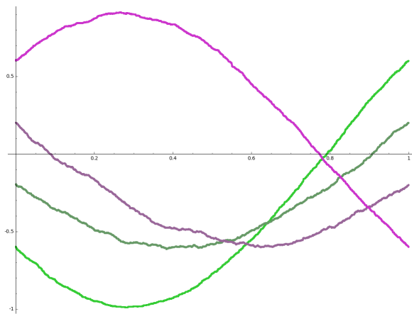
FIGURE 5. The scaled trajectories of the elements 200, 400, 600 and 800 in a 1000-element random sorting network.
