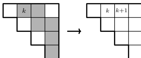
FIGURE 20. The bijection in the proof of Theorem 6.3 with k = k(T) and the path of \tau_{k(T)} \circ \dots \circ \tau_{|\lambda|-1} coloured.
