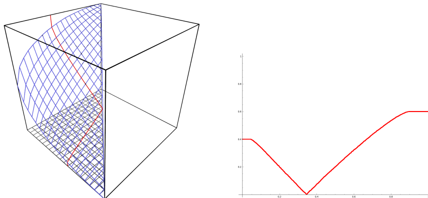
FIGURE 17. A curve (in red) determining the trajectory of \lfloor \beta n \rfloor , \beta = 0.4 , shown on the right from the limit shape.
