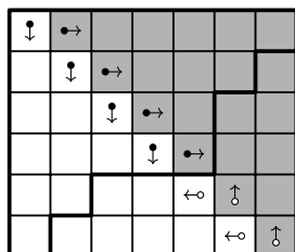
FIGURE 10. The partition \square_7 = (7^6) . The shifted diagram of \lambda = (6, 4, 2, 1) is in grey in the upper left part, which is the diagram of \Lambda = (7, 6, 5, 5, 2, 1) . The diagram of \square_7 \setminus \Lambda = (6, 5, 2, 2, 1) is a 180° rotation of the lower right part. The shifted diagram of \Delta_7 \setminus \lambda = (5, 3) is the reflection through the diagonal i = j of the grey region in the lower right part. The partition \square_7 \setminus \Lambda = (6, 5, 2, 2, 1) is the double of \Delta_7 \setminus \lambda .
