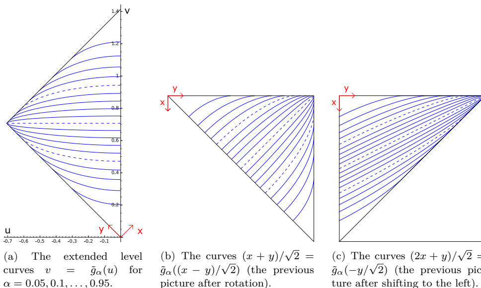
FIGURE 13. Translating the limit shape of shifted staircase SYT into the limit of the diagrams of the intermediate permutations. The blue curves in (c) are the limit curves of the diagrams of the intermediate permutations at times \alpha = 0.05, 0.1, \dots, 0.95 . The dashed curves correspond to the values \alpha = 0.25, 0.5 and 0.75 , and also appear in Figure 14.
