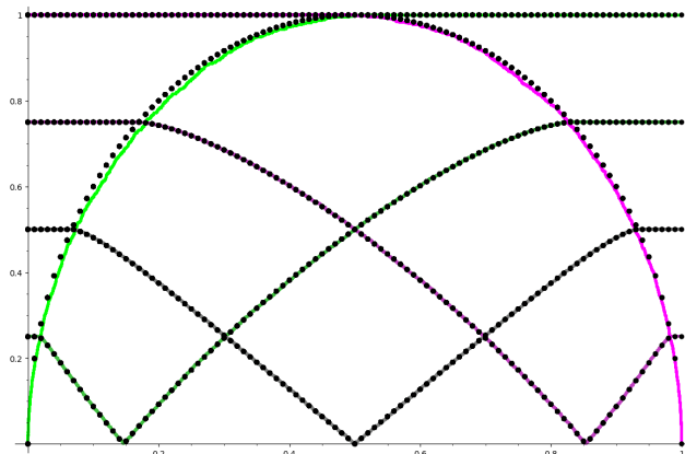
FIGURE 16. The scaled trajectories of the elements 1, 250, 500, 750 and 1000 in a random 132-avoiding sorting network with 1000 elements together with points (in black) from their limits in Theorem 5.4. Compare with Figure 5.
