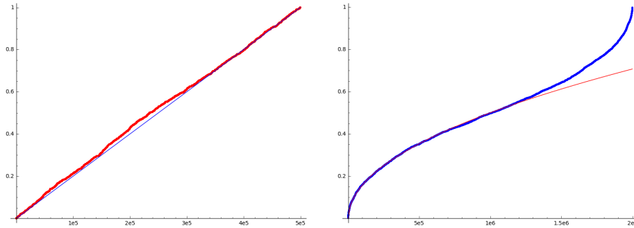
FIGURE 21. The number of adjacencies in an initial segment of a random sorting network of size n = 1000 , (left) seems to grow linearly. The number of adjacencies in an initial segment of a random 132-avoiding sorting network of size n = 2000 (right) seems to grow like a square root for the first half.
