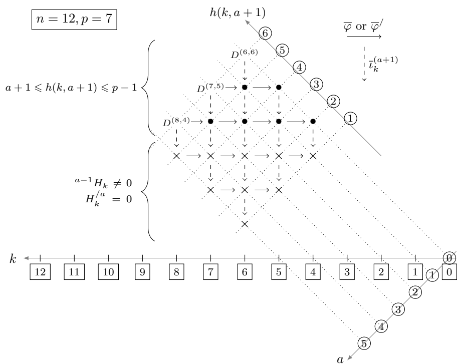
FIGURE 1. Positions of non-vanishing homology groups for (n, p) = (12, 7) .
