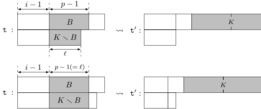
FIGURE 2. Notations used in Lemma 5.17.
