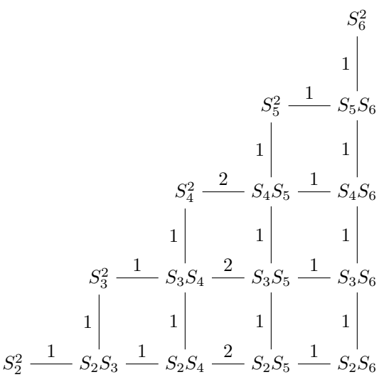
FIGURE 2. n = 6 and j_0 = 4 for the P -index
