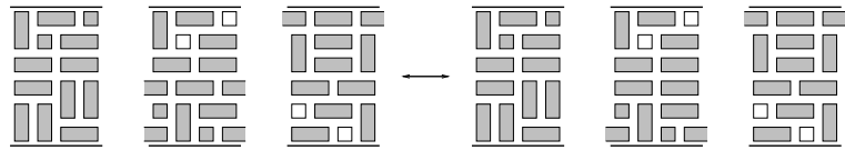
FIGURE 6. Two tilings of \hat{\mathcal{R}}_N for N = 3 and L = 6 . The two tilings differ by a pseudoflip in the fourth row of the second floor.
