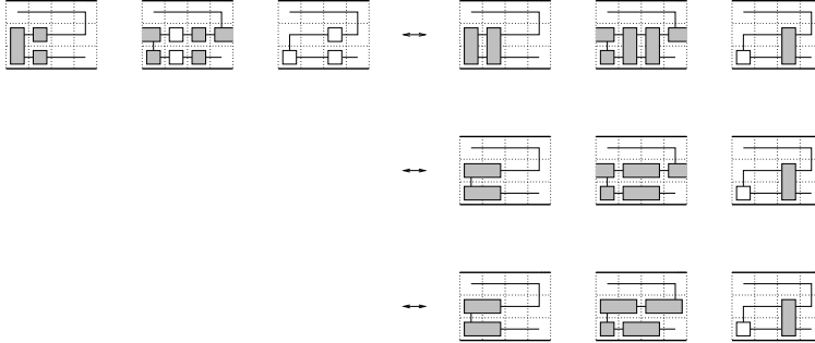
FIGURE 13. The case |\phi_0| = 1 .
