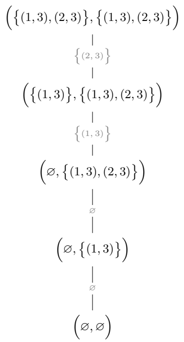
Figure 3. The poset (\mathbf{NN}_{3;2}^{(2)}, \subseteq) .
