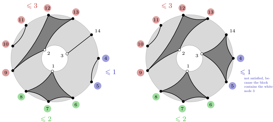
(a) The annular diagram of the non-crossing 3-partition from Figure 1a.
