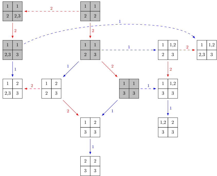
FIGURE 2. The K-crystal for SV^3\left(\begin{smallmatrix} \square & \square \\ \square & \square \end{smallmatrix}\right) with the K-crystal operators depicted by dashed lines. The K-Demazure crystal B_{s_2} is the restriction to the subset of shaded tableaux.
