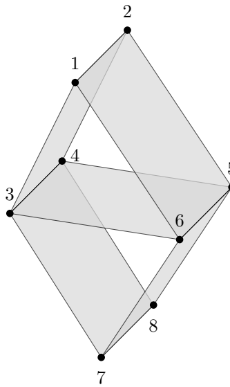
FIGURE 1. A visual representation of the circuit-hyperplanes for V .
