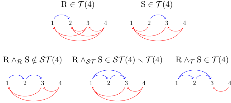
FIGURE 4. Two transitive relations R, S \in \mathcal{T}(4) (top) and their meets R \wedge_{\mathcal{R}} S , R \wedge_{\mathcal{ST}} S and R \wedge_{\mathcal{T}} S (bottom).
