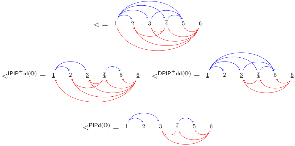
FIGURE 21. The \text{IPIP}^\pm(\mathbb{O}) increasing deletion, the \text{DPIP}^\pm(\mathbb{O}) decreasing deletion, and the \text{PIP}(\mathbb{O}) deletion.
