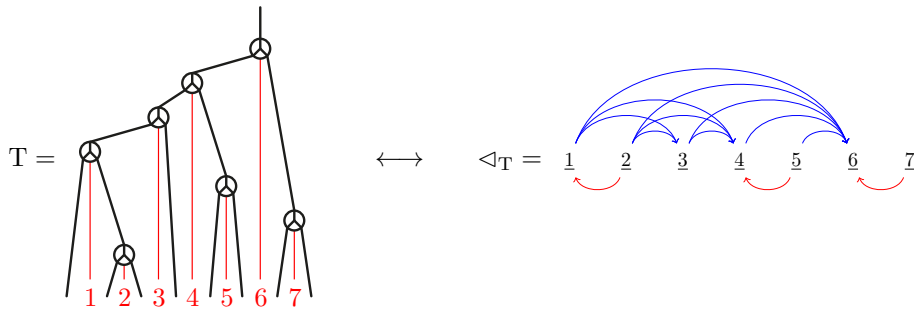
FIGURE 11. A Tamari Order Element Poset (TOEP).
