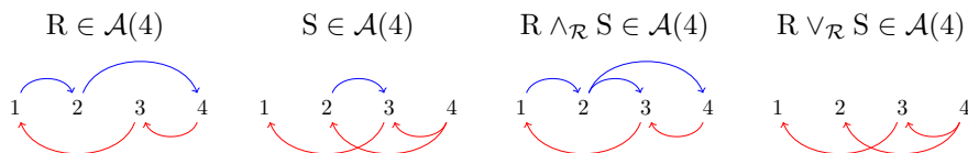
FIGURE 2. Two antisymmetric relations R, S \in \mathcal{A}(4) (left) and their meet R \wedge_{\mathcal{R}} S and join R \vee_{\mathcal{R}} S (right).
