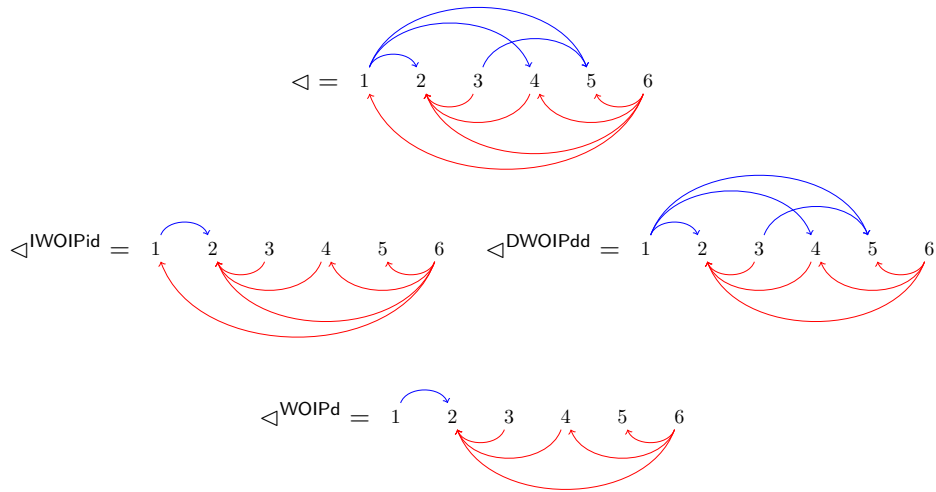
FIGURE 10. The IWOIP increasing deletion, the DWOIP decreasing deletion, and the WOIP deletion.
