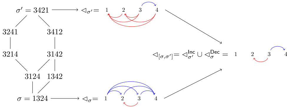
FIGURE 7. A Weak Order Interval Poset (WOIP).
