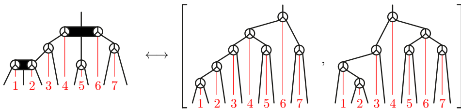
FIGURE 13. A Schröder tree S (left) can be seen as an interval [\mathsf{T}^{\min}(S), \mathsf{T}^{\max}(S)] in the Tamari lattice (right).
