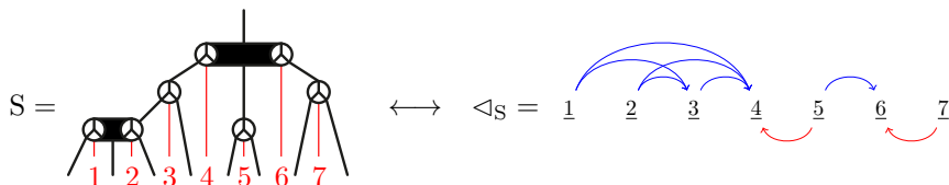
FIGURE 14. A Tamari Order Face Poset (TOFP).
