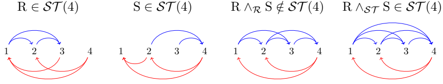
FIGURE 3. Two semi-transitive relations R, S \in \mathcal{ST}(4) (left) and their meets R \wedge_{\mathcal{R}} S and R \wedge_{\mathcal{ST}} S (right).
