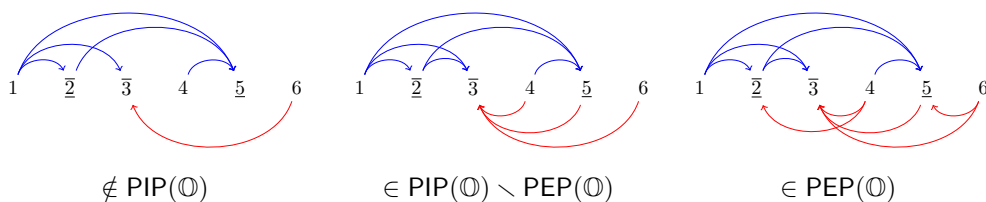
FIGURE 16. Examples and counterexamples of elements in \text{PIP}(\mathbb{O}) and \text{PEP}(\mathbb{O}) , where \mathbb{O} = (6, \{2, 3\}, \{2, 5\}) .
