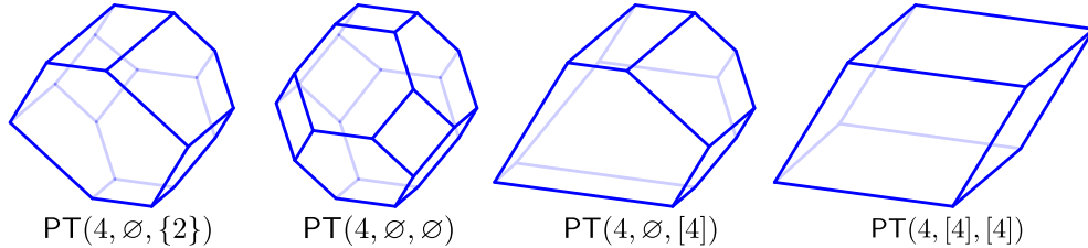
FIGURE 18. Four examples of permutreehedra. While the first is generic, the last three are a permutahedron, an associahedron [9], and a parallelepiped.
