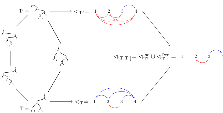
FIGURE 12. A Tamari Order Interval Poset (TOIP).
