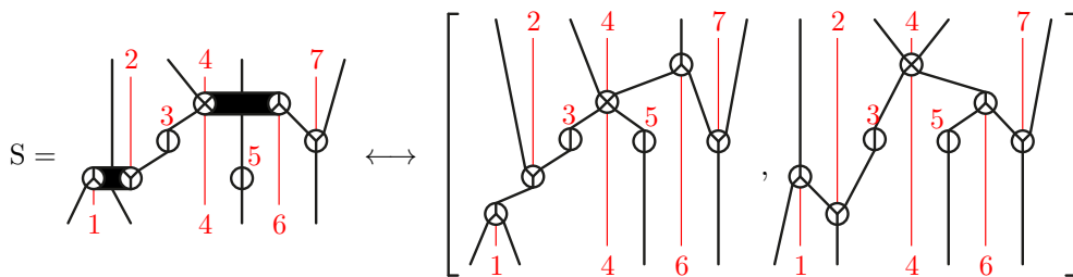
FIGURE 20. A Schröder permutree S (left) can be seen as an interval [T^{\min}(S), T^{\max}(S)] in the permutree lattice (right).
