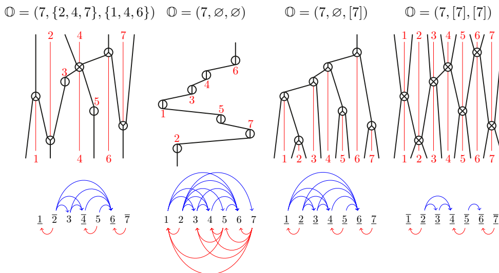
FIGURE 15. Four examples of permutrees T (top) with their posets \triangleleft_T (bottom). While the first is generic, the last three illustrate specific orientations corresponding to permutations, binary trees, and binary sequences.
