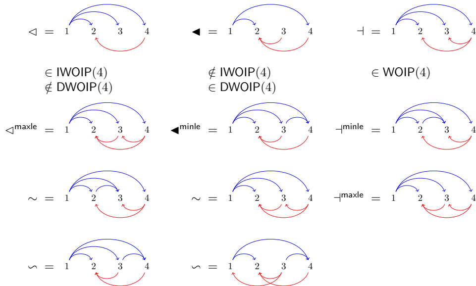
FIGURE 9. Examples and counterexamples of elements in \text{IWOIP}(4) and \text{DWOIP}(4) .
