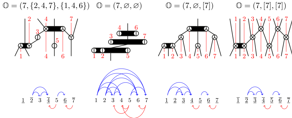
FIGURE 19. Four examples of Schröder permutrees S (top) with their posets \triangleleft_S (bottom). While the first is generic, the last three illustrate specific orientations corresponding to ordered partitions, Schröder trees, Schröder Cambrian trees, and ternary sequences.
