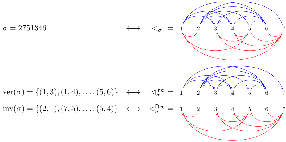
FIGURE 6. A Weak Order Element Poset (WOEP).
