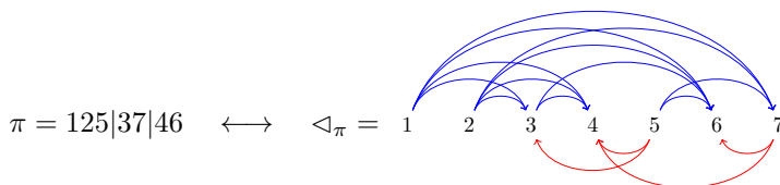
FIGURE 8. A Weak Order Face Poset (WOFP).
