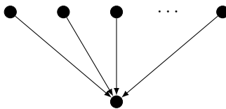
FIGURE 5. An n -fan.
