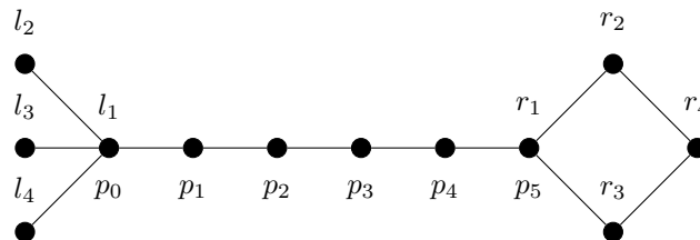
FIGURE 2. The graph K_{3,1} \oplus_4 C_4 .
