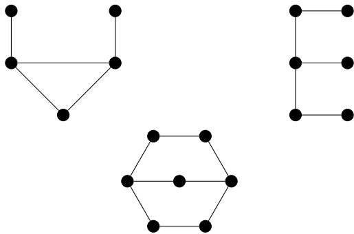
FIGURE 4. The bull graph (left), E-graph (right) and \theta_0 graph (below).
