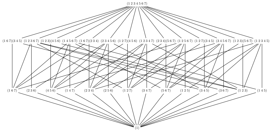
FIGURE 1. The poset ONC_7 = (ONC_7, \leq_3) .
