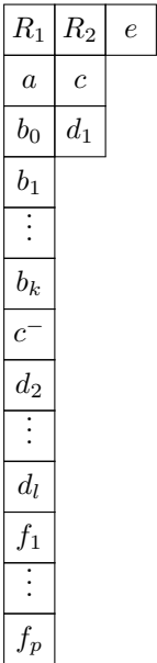
FIGURE 1. The insertion tableau for \sigma' in Case 1.
