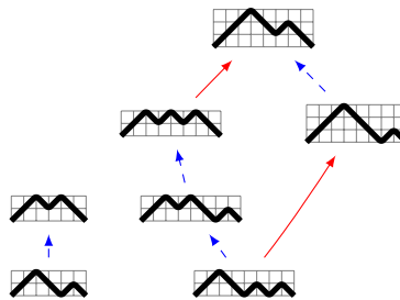
FIGURE 10. The Hochschild intervals F_1 and F_2 .
